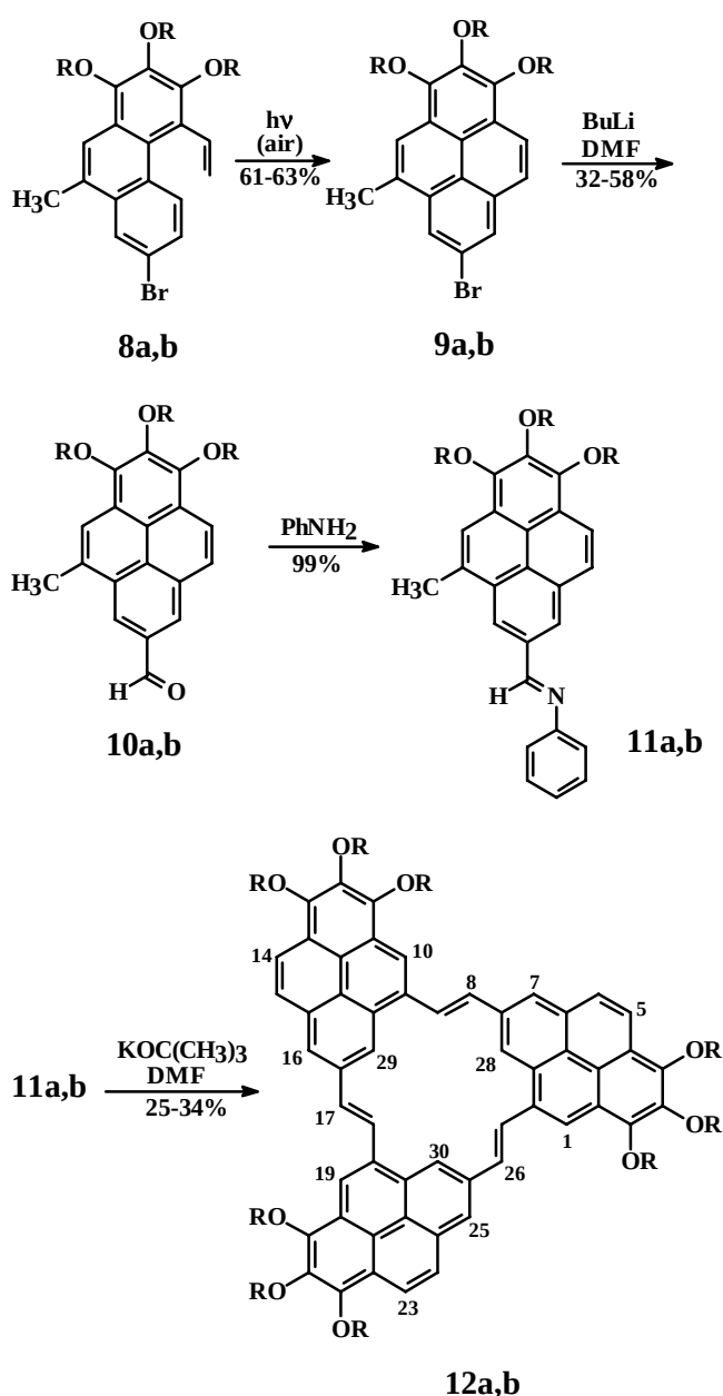
Scheme 1 Preparation of the tripyreno[18]annulenes 12a,b
